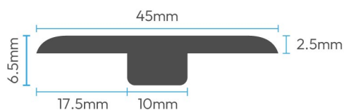
SPC T Profile
