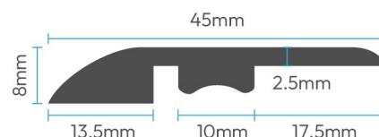
SPC A Profile
