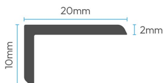
SPC L Profile
