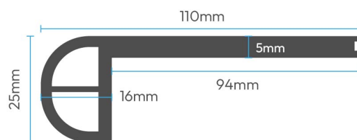
SPC Flush Nosing
